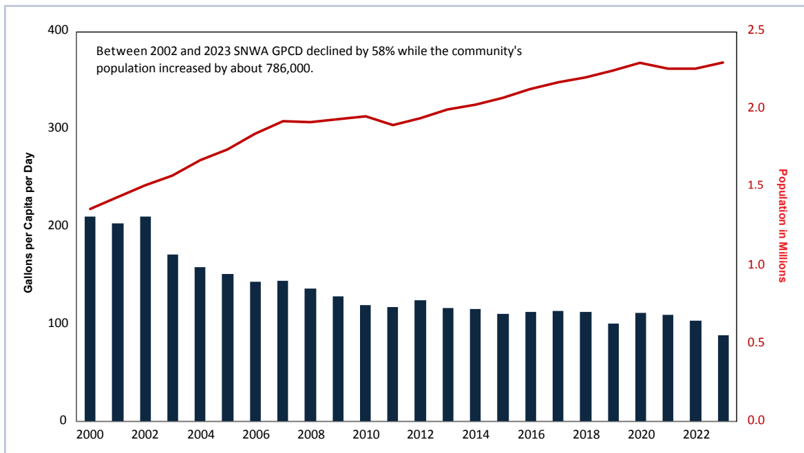
FIGURE 3.4 Population & Per Capita Water Use
