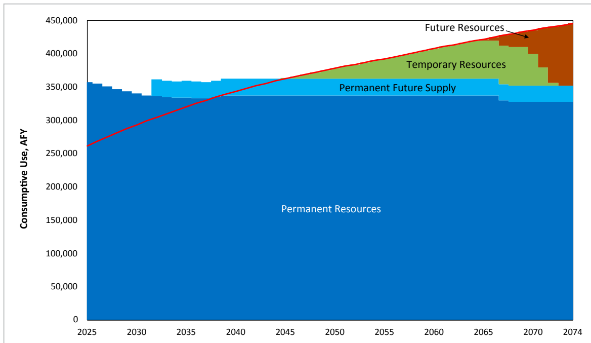
FIGURE 4.13 11.0 MAFY Natural Flow, Upper Demand (92 GPCD by 2055)
