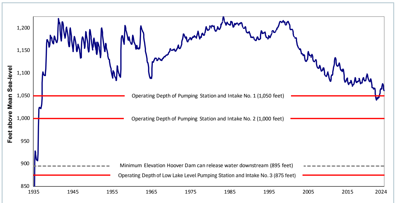
FIGURE 2.6 Historical Lake Mead Elevations
