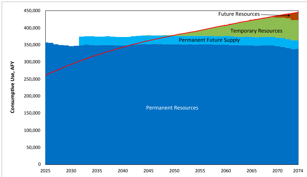
FIGURE 4.9 13.3 MAFY Natural Flow, Upper Demand (92 GPCD by 2055)
